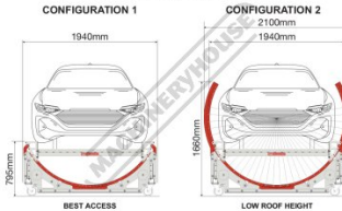
Modular Design Configurations 1-2
