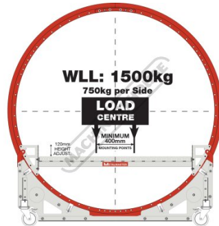
1500kg Total Capacity 750kg Per Side
