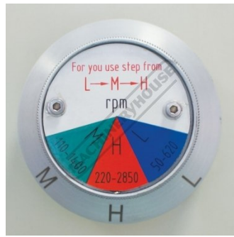
3 Speed Gearbox
