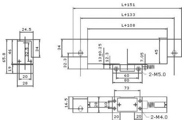
GS20 Series from 1300mm to 3000mm
