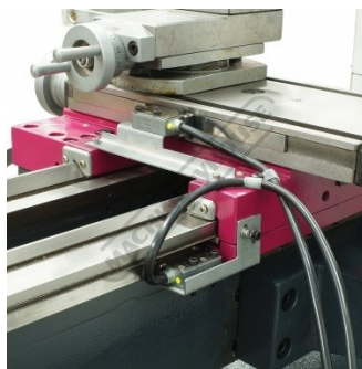
Shown with Optional 2 Axis DRO Scales
