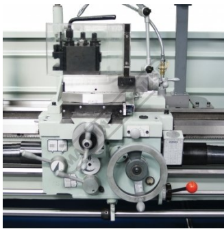
Saddle Controls
