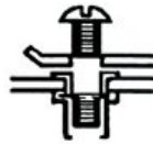
Figure3 Remove tool this is your Finished Rivet Nut installation
