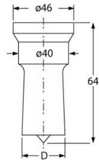
Punches 32, 38, 40
