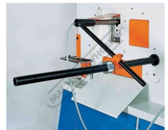
Includes Auto Touch & Cut Length Stop
