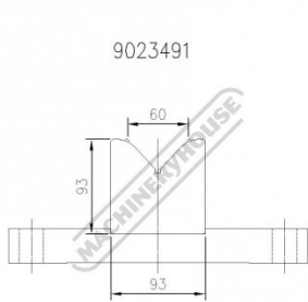
Single Vee Pressbrake Diagram
