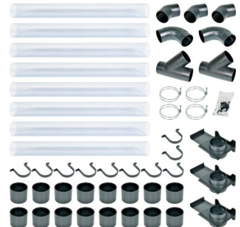
W3447 Wall Mounted Wood Dust Extraction Ducting Kit
