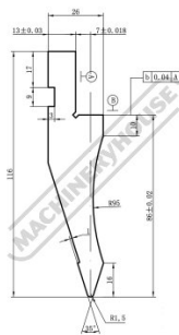
Top Tooling Diagram
