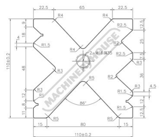
Multi V Die Block - 4mm-80mm
