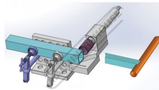
Square Tubes
