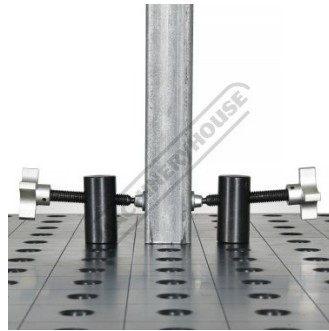
Clamp Position
